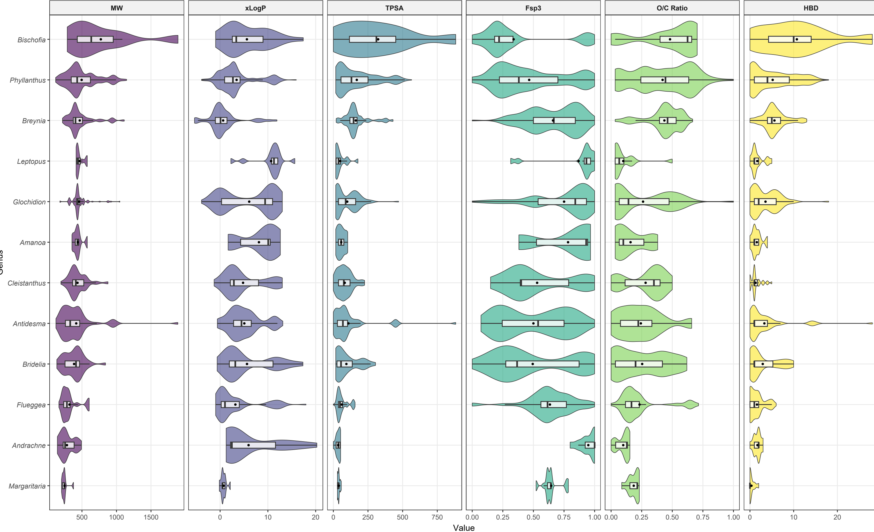
Physicochemical Distributions (Inc. O/C) — Phyllanthaceae
