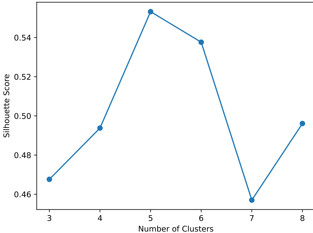
KMeans income_spending Silhouette Method
