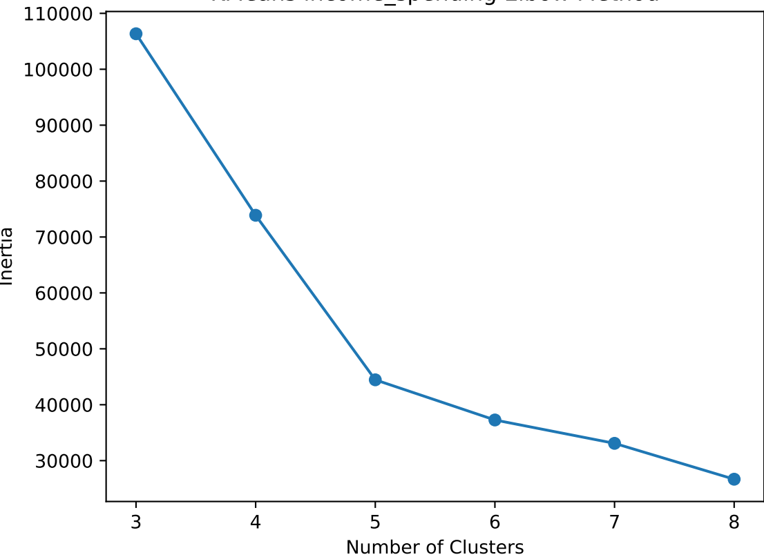
KMeans income_spending Elbow Method
