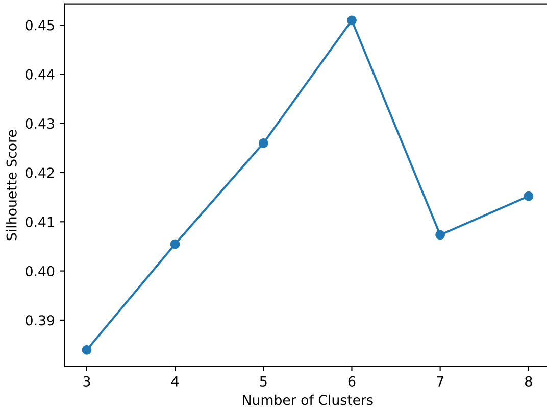
KMeans income_spending_age Silhouette Method
