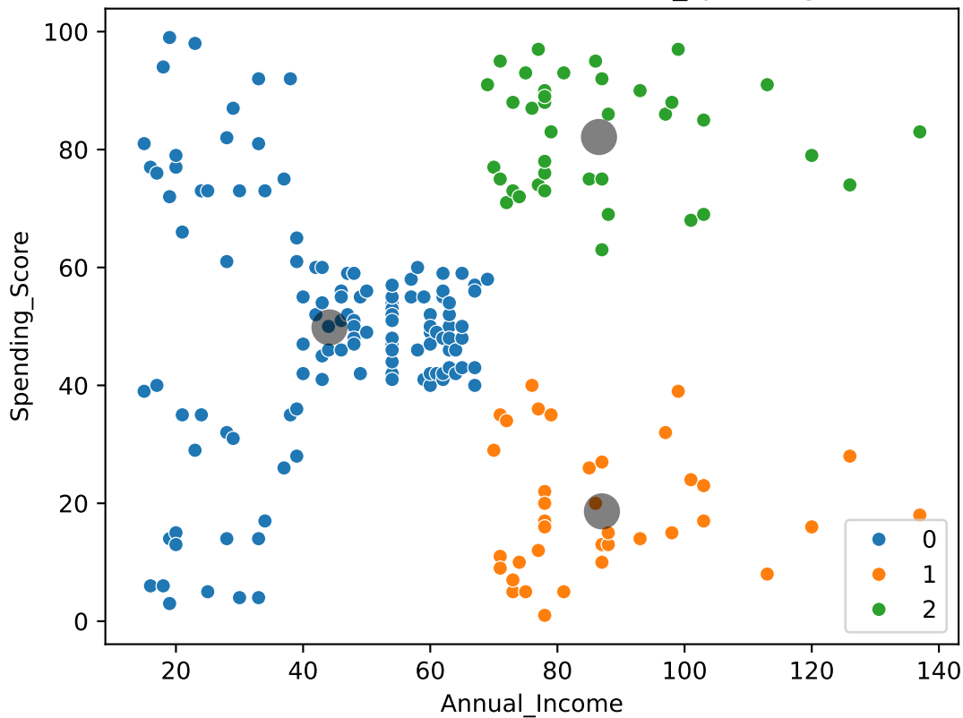
KMeans 3 Clusters for income_spending
