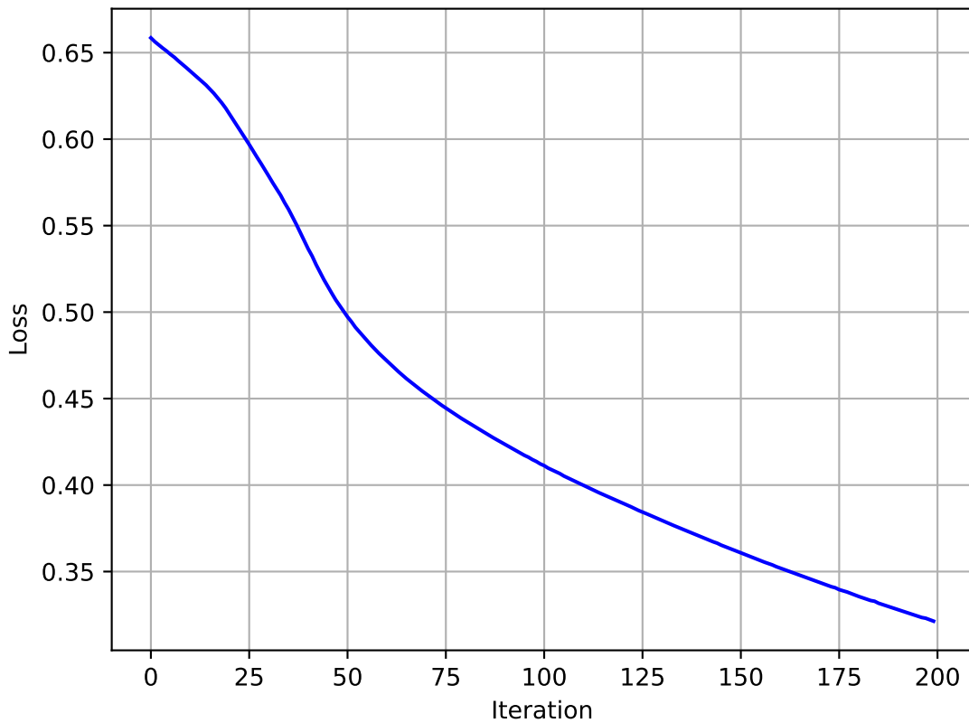
Activation: relu
