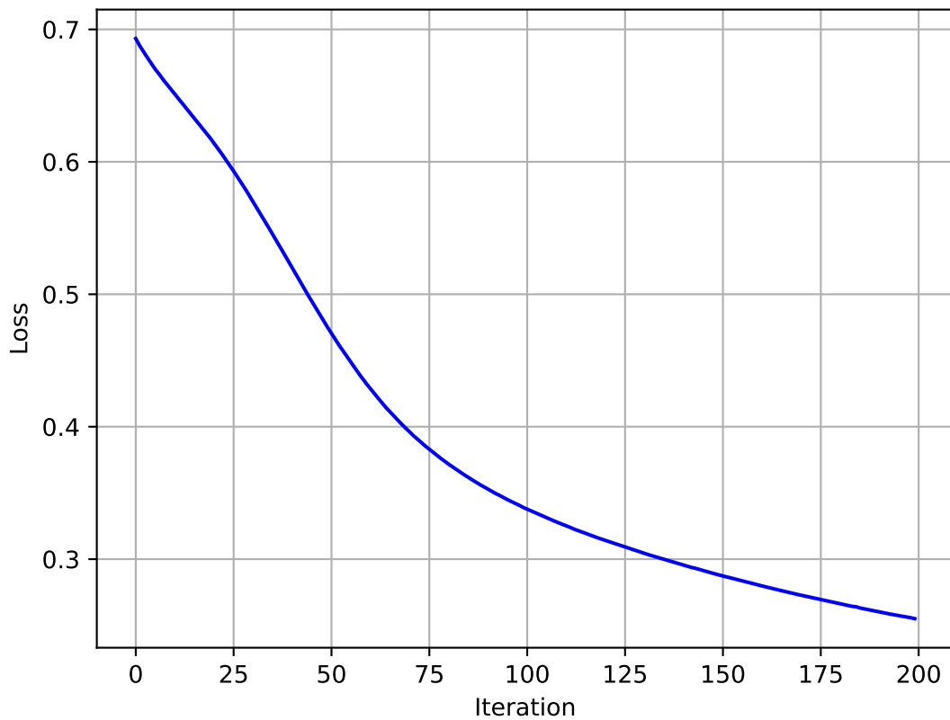
Activation: tanh
