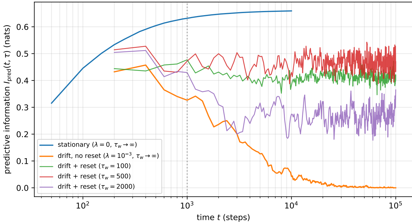
Collapse vs retention of I_{\text{pred}}(t) ( k=8 , \tau=1 , \lambda=10^{-3} )
