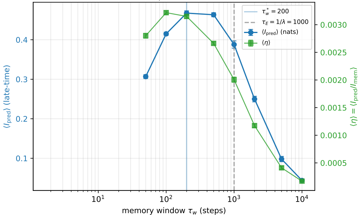
Optimal forgetting: \langle I_{\text{pred}} \rangle vs \tau_w at \lambda = 10^{-3} ( k=8 )
