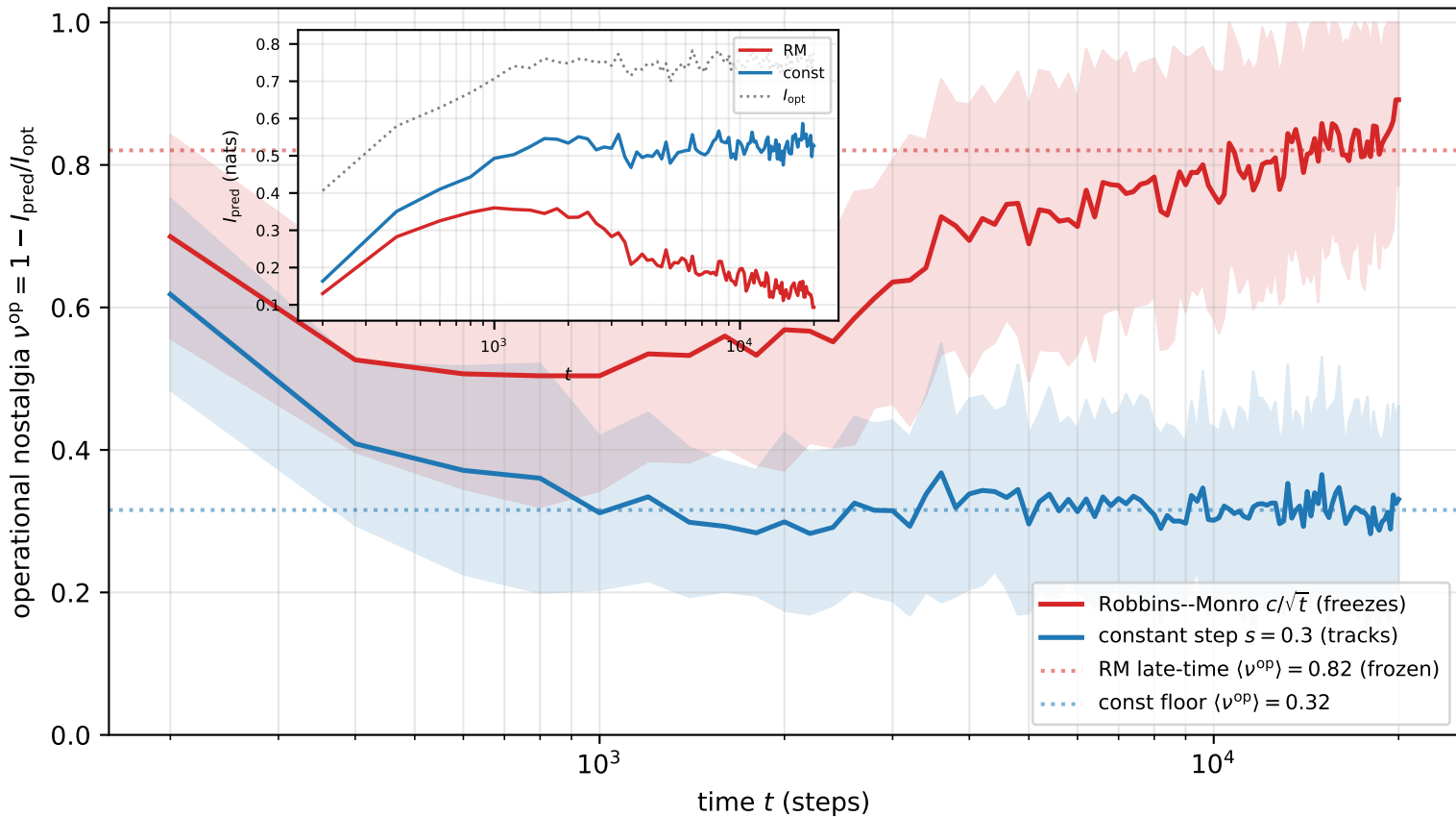
Freezing vs tracking under drift: \nu^{\text{op}}(t) ( k = 8 , \lambda = 0.001 , \sigma = 0.1 )
