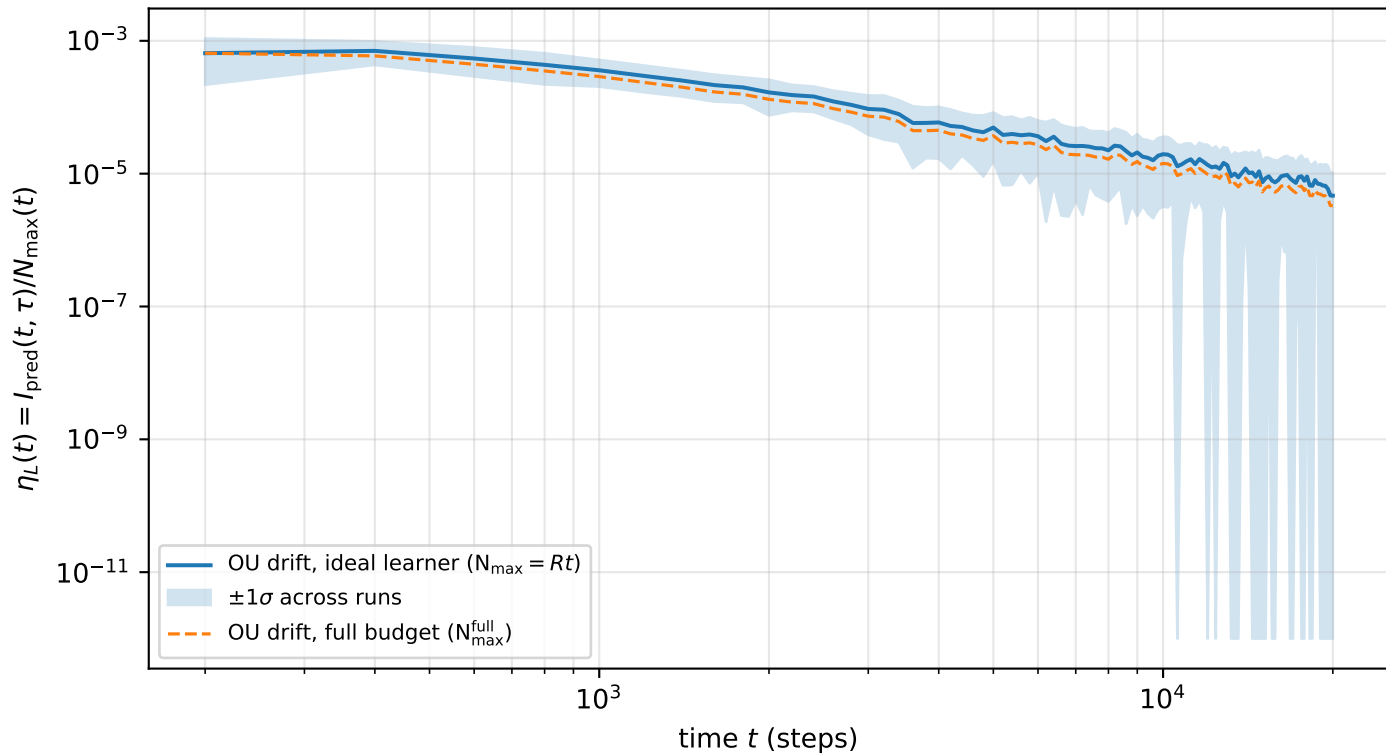
OU drift: \eta_L(t) averaged over 50 runs ( k = 8, \lambda = 0.001, \sigma = 0.1 )
