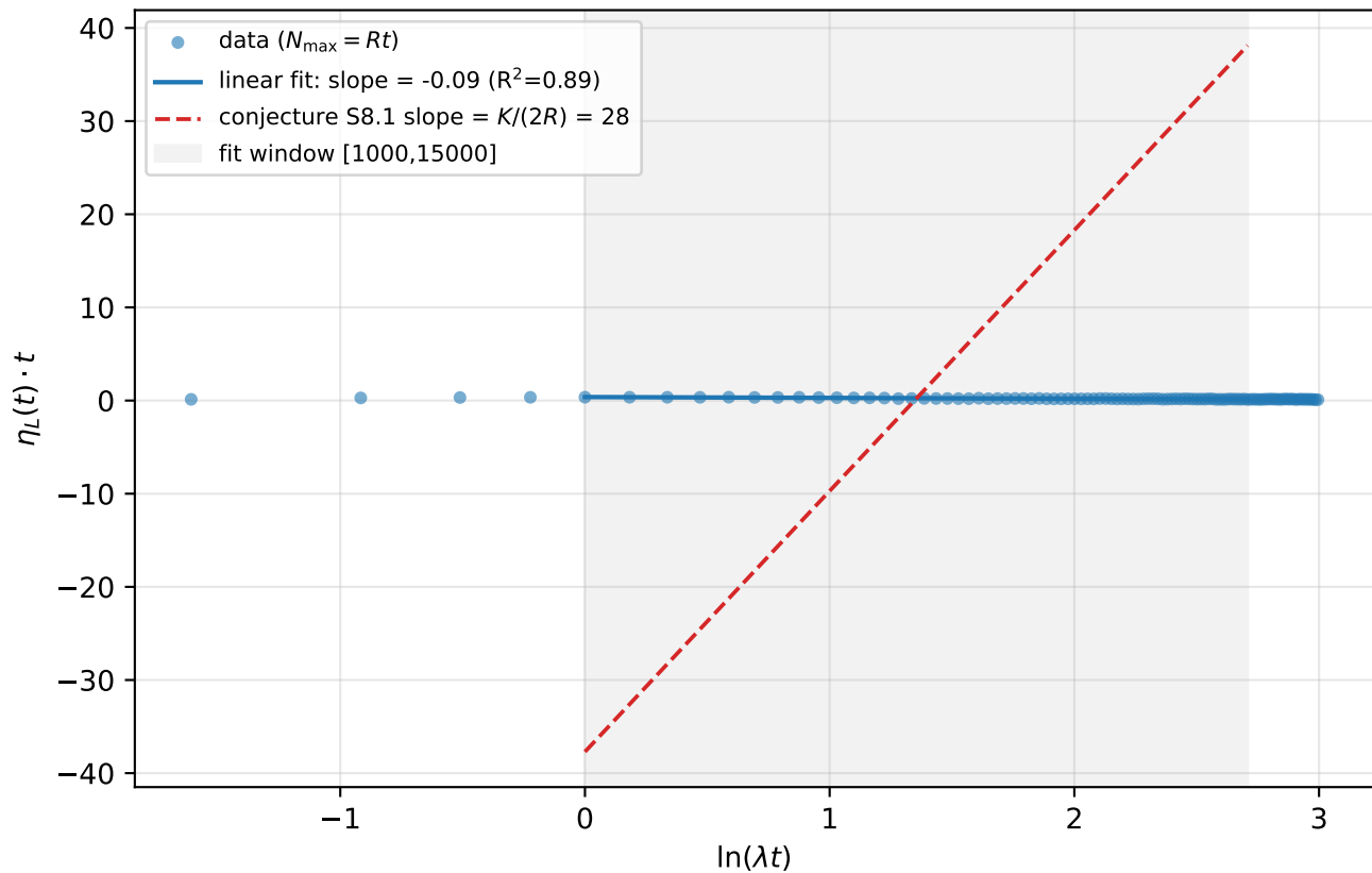
Check of conjecture S8.1 / (S8.2): \eta_L \cdot t vs \ln(\lambda t) (OU class)
