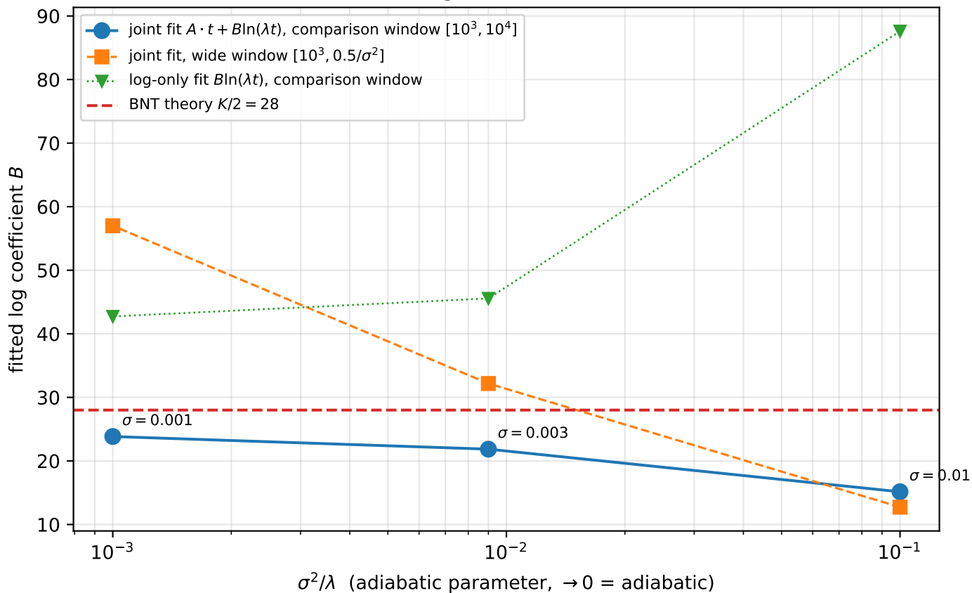
Adiabatic scan: BNT log-coefficient B vs \sigma^2/\lambda ( N_{\text{runs}} = 25 )
