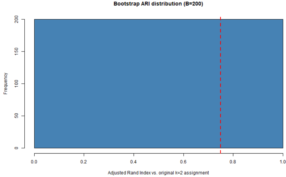
Figure 10: Bootstrap-ARI distribution (B=200) for the k=2 country clustering (H6). Dashed line: pre-registered threshold of 0.75.
