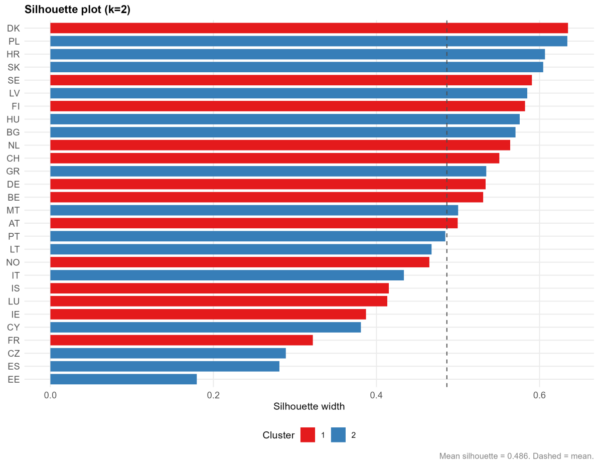
Figure 14: Silhouette plot (k=2): per-country silhouette widths.
