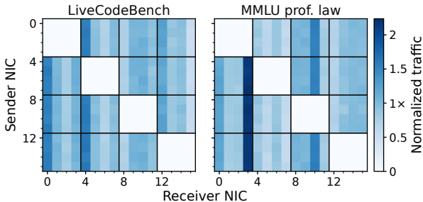
(c) NIC-to-NIC dispatch traffic
