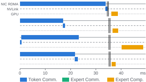
Computation Imbalance+ Communication Imbalance
