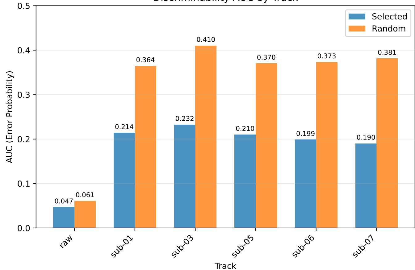
Discriminability AUC by Track
