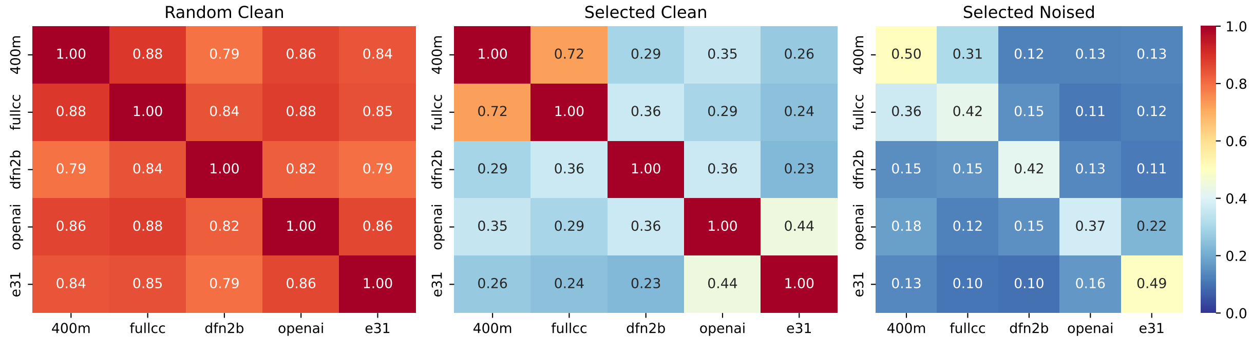
Correlation Matrices: sub-05
