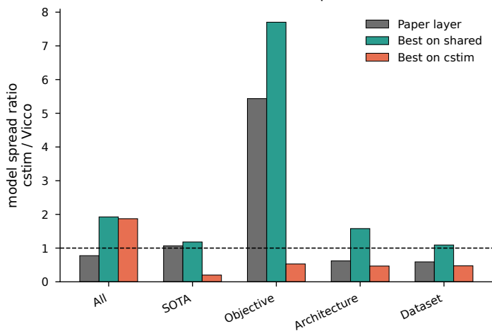
Between-model spread
