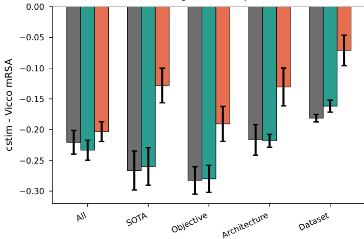
Alignment drop
