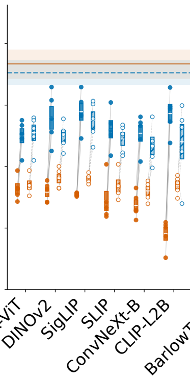
b State of the Art
