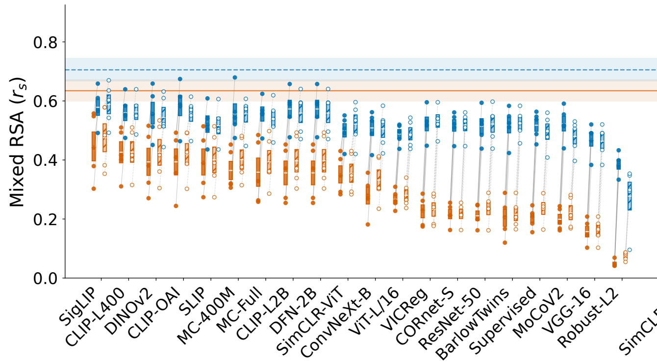
a All Models
