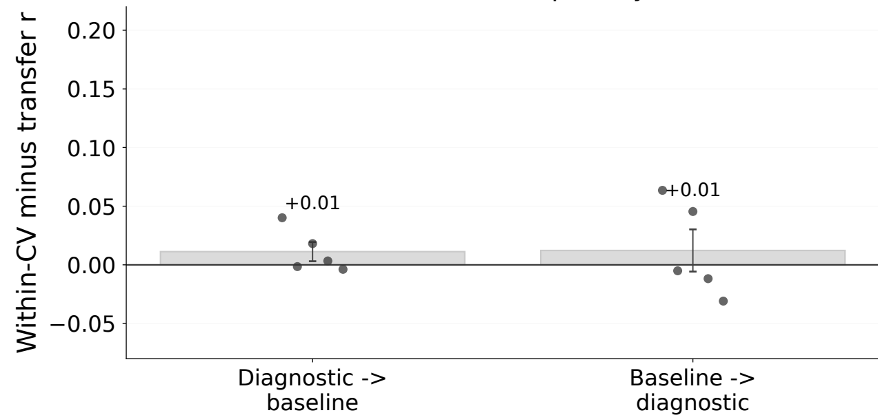
Model-ensemble weights do not remove the diagnostic gap across stimulus regimes Mixed ensemble transfer
