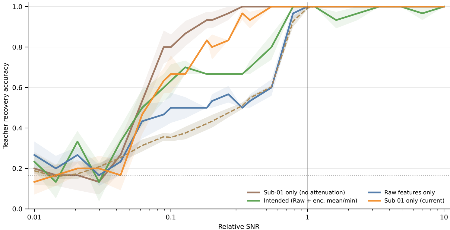
Independent-refit teacher/student recovery (encoded, 1k refit)
