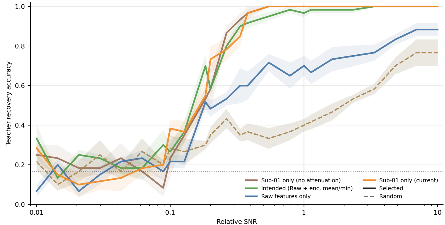
Teacher/student fitted-recovery curves (encoded)
