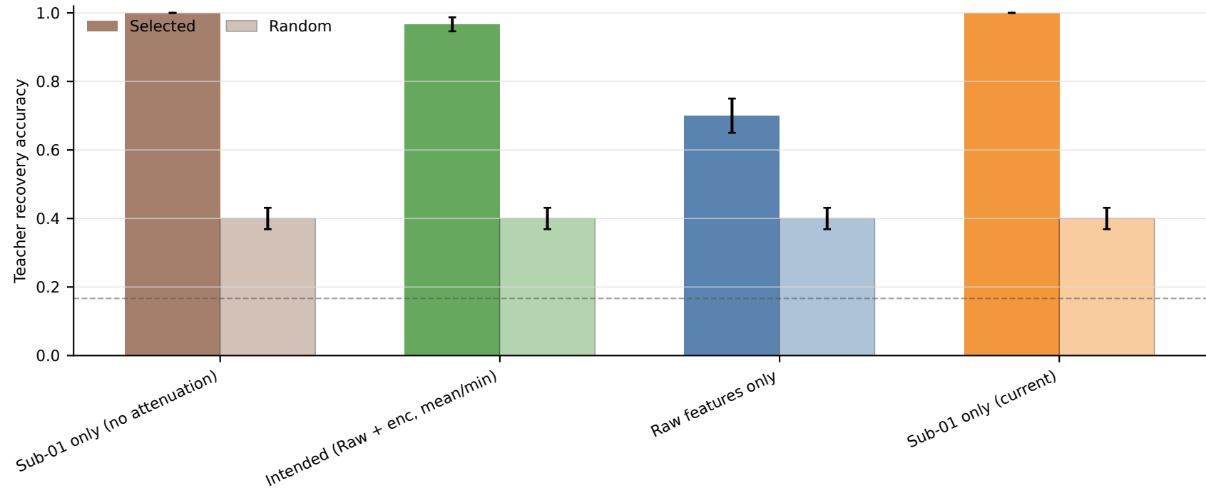
Teacher/student fitted recovery (encoded) at noise x1
