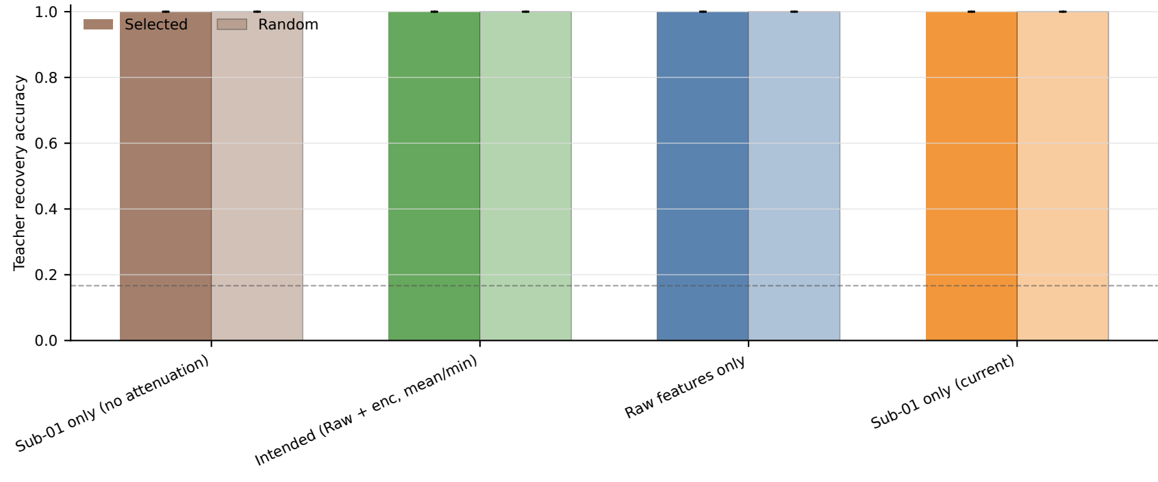
Teacher/student fitted recovery (raw) at noise x1
