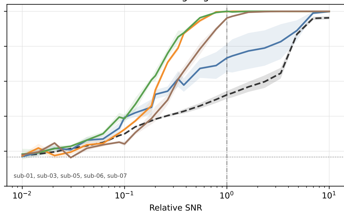
Encoding avg
