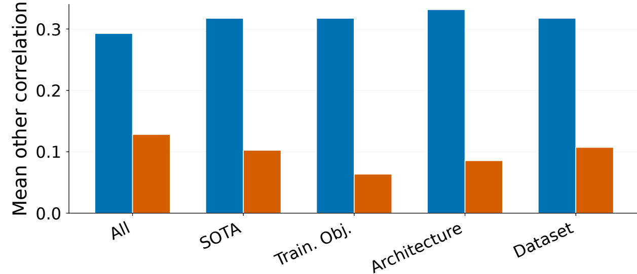
Absolute other-correlation
