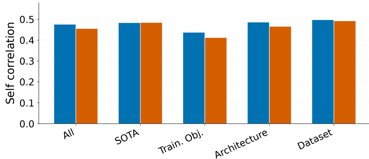
Absolute self-correlation
