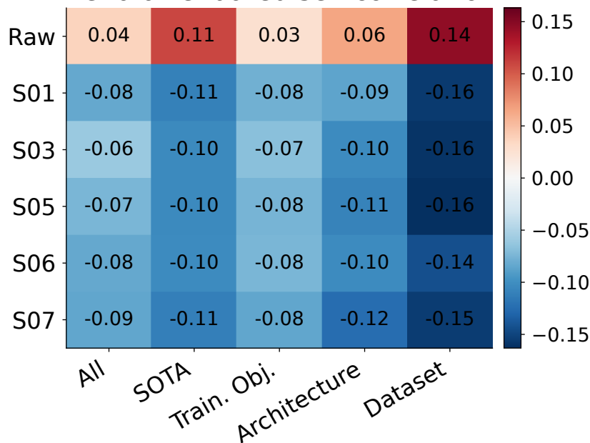
Delta attenuated self-correlation
