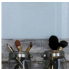
*robustness_imagenet_l2_eps3 energy=0.778
