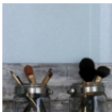
torchvision_resnet50_imagenet1k_v1 energy=0.603
