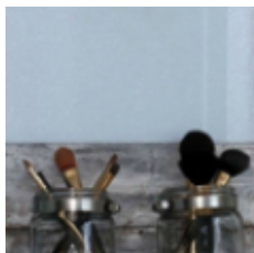
slip_vit_l_slip energy=0.502
