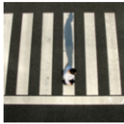
dinov2_vitl14 query
