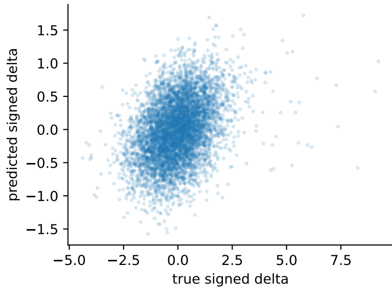
Signed disagreement
