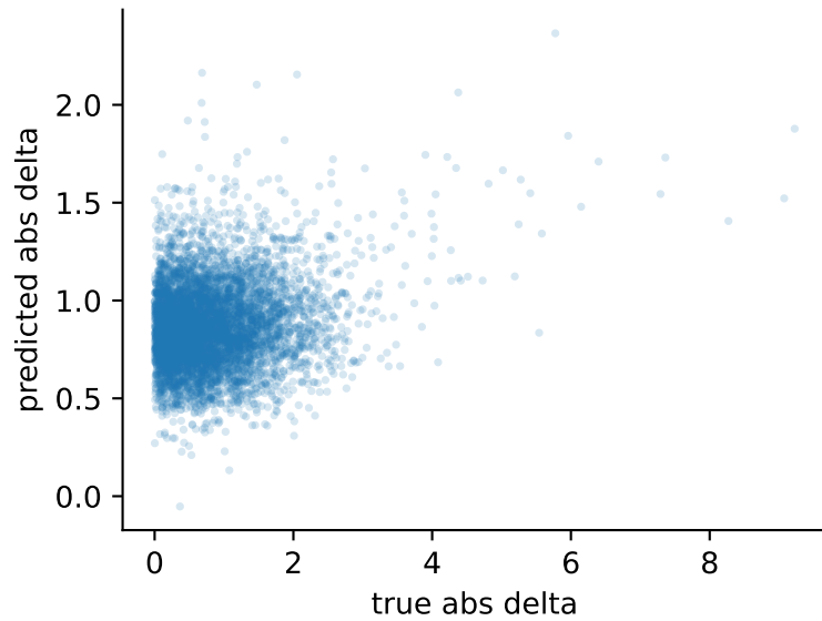
Absolute disagreement
