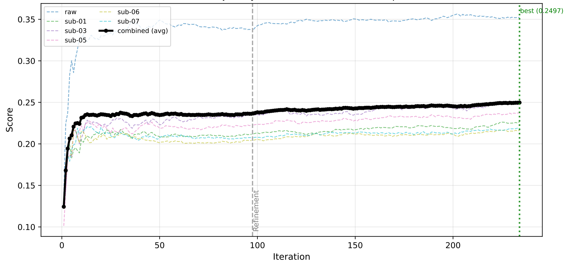
Selection Score Trajectory (Raw) (+ 137 refinement replacements)
