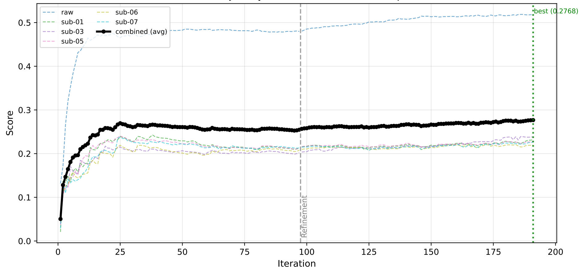
Selection Score Trajectory (Raw) (+ 94 refinement replacements)
