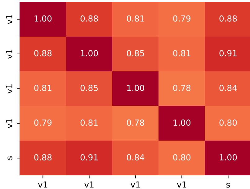
Random Clean
