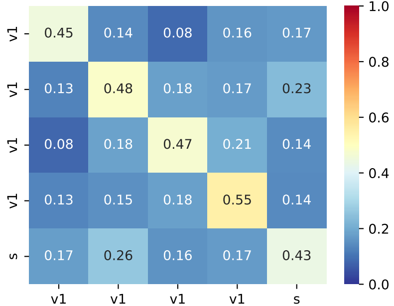
Selected Noised
