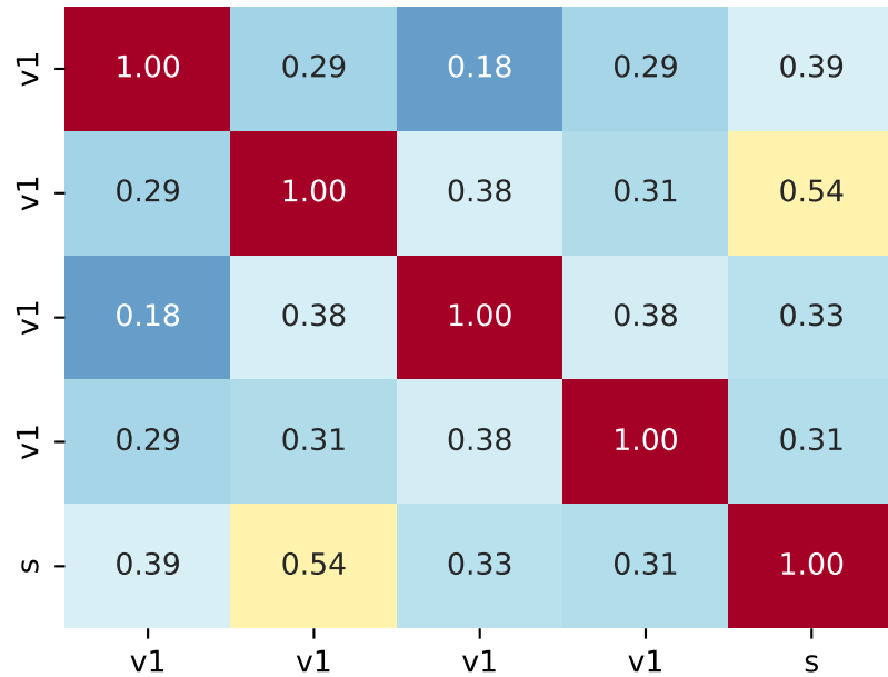
Selected Clean
