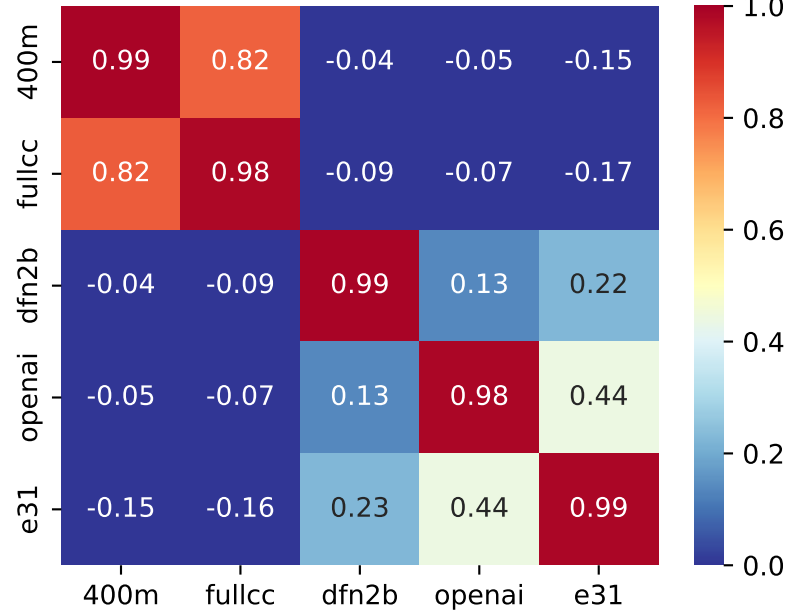
Selected Noised
