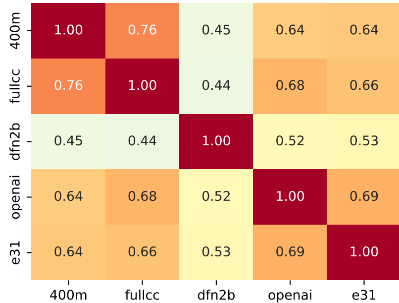
Random Clean
