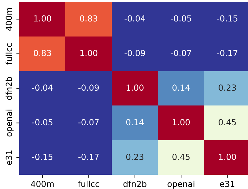
Selected Clean
