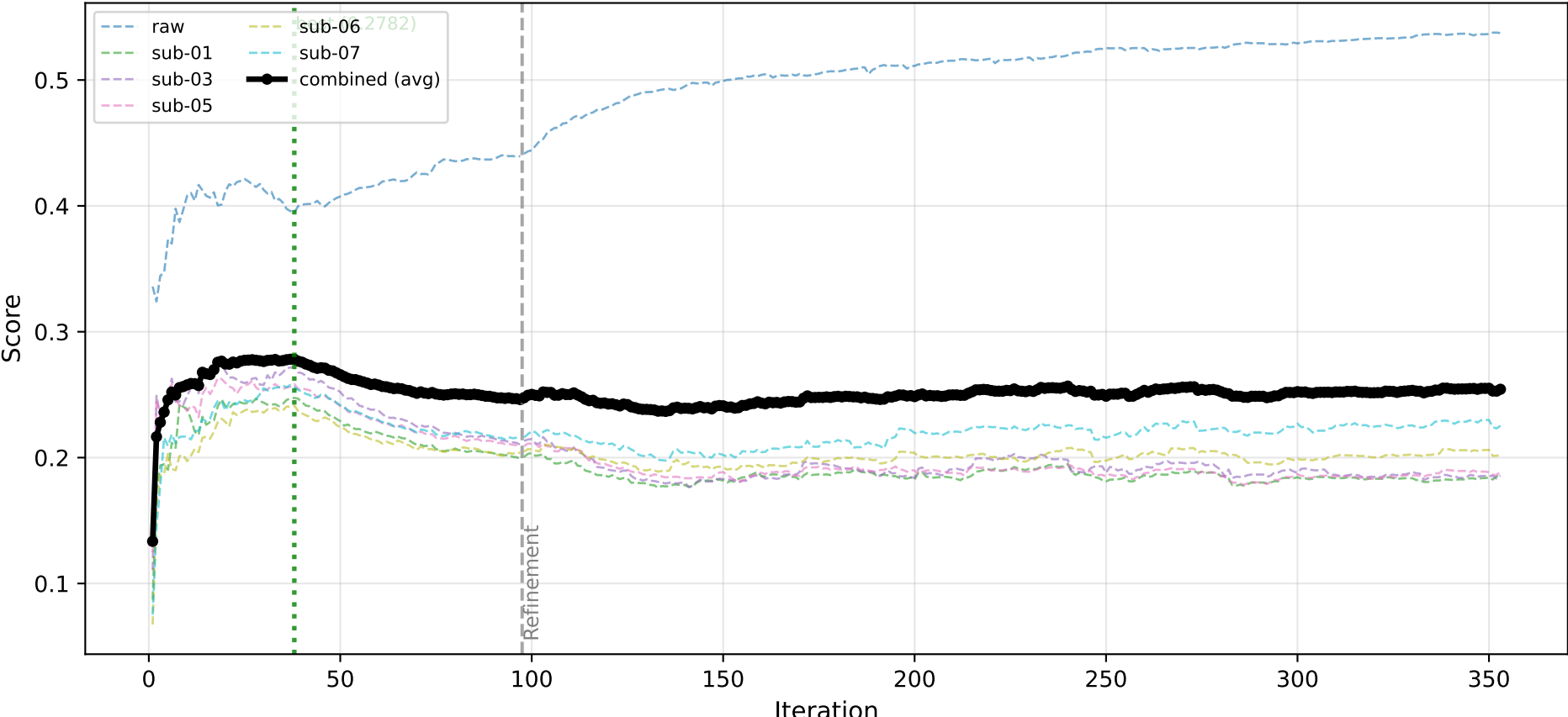
Selection Score Trajectory (Raw) (+ 256 refinement replacements)
