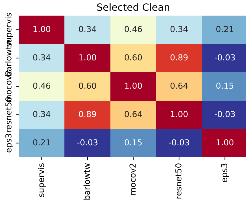
Correlation Matrices: sub-06
