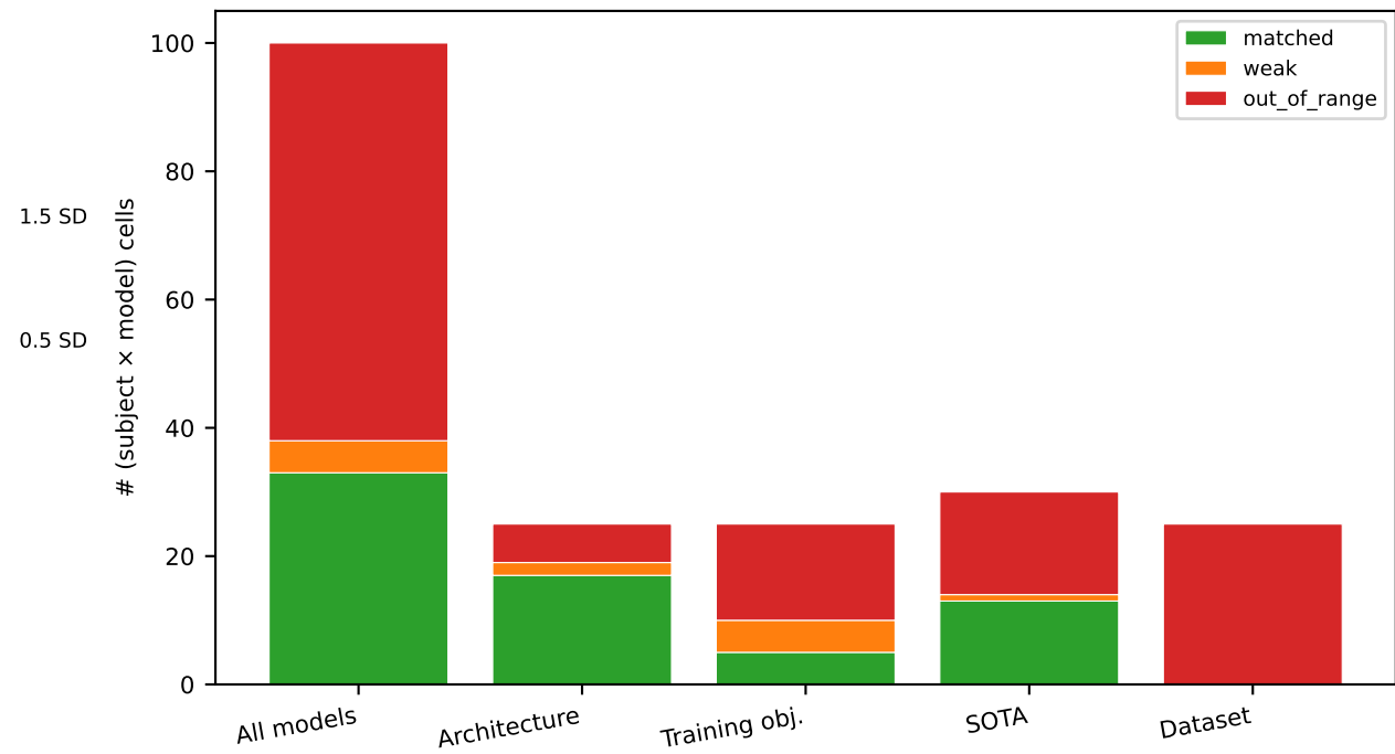
Match-quality cell counts (out of 25–100 per set)
