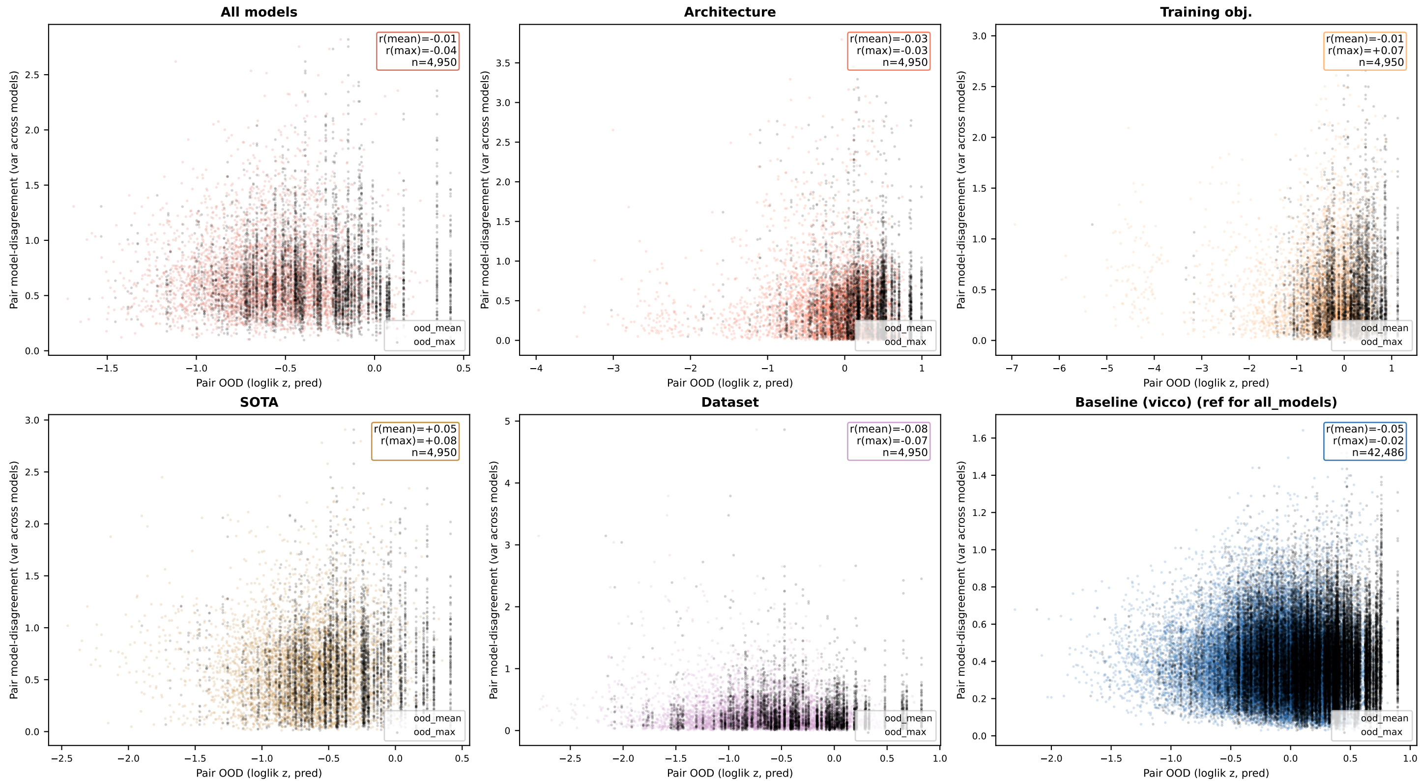
Pair-level disagreement vs OOD (per-set model rosters; both ood_mean and ood_max)
