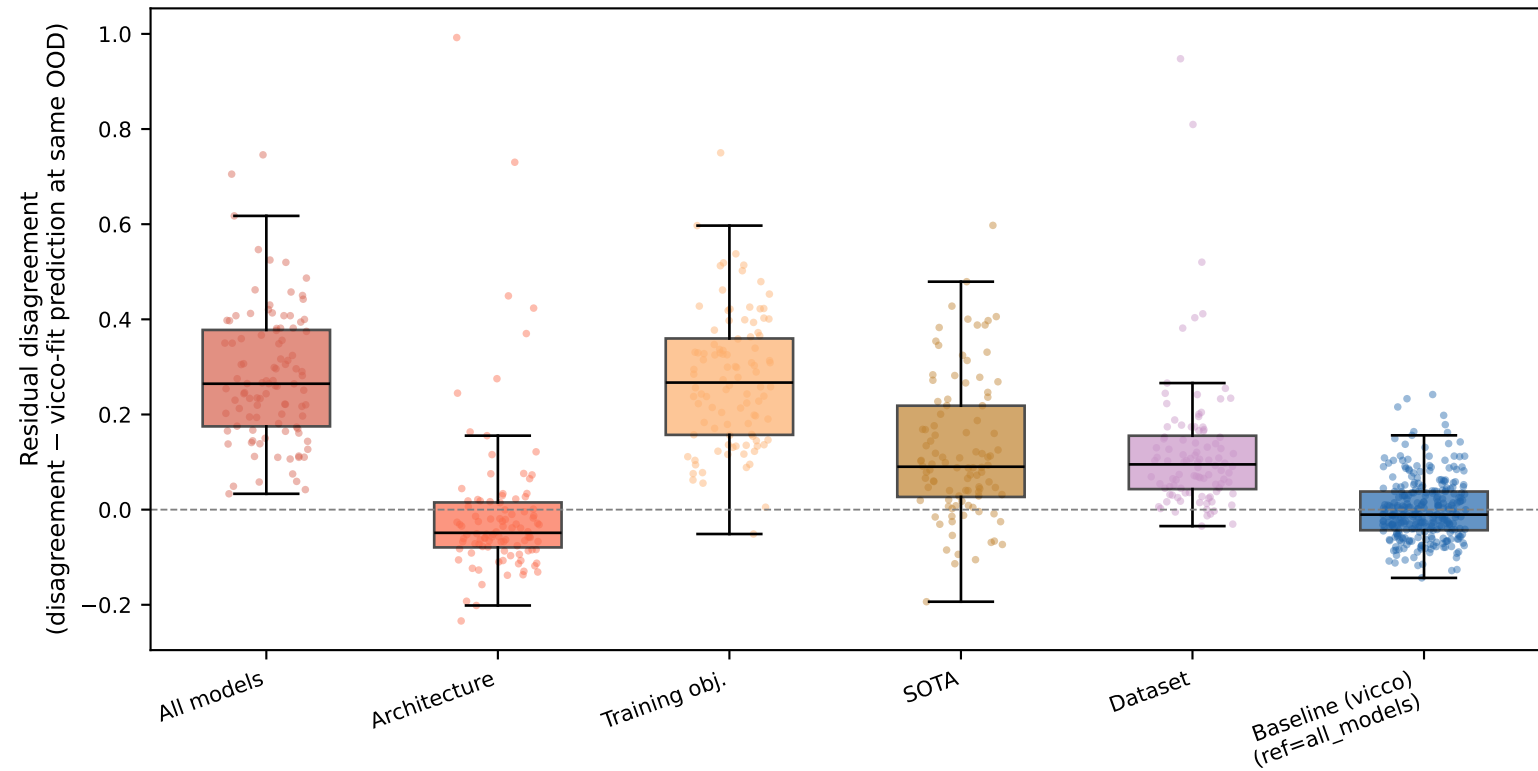
Residual model-disagreement at matched OOD Each set's residual uses a vicco reference fit on the SAME model roster
