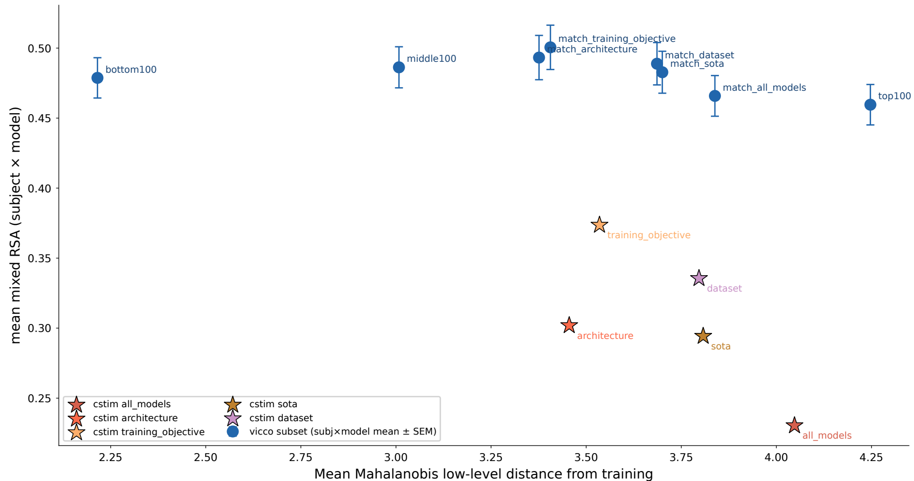
Mixed RSA on vicco subsets spanning the low-level distance range, vs. cstim sets at their respective mean low-level distances
