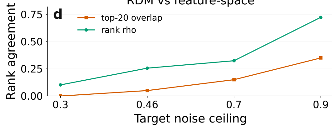
Candidate rankings RDM vs feature-space
