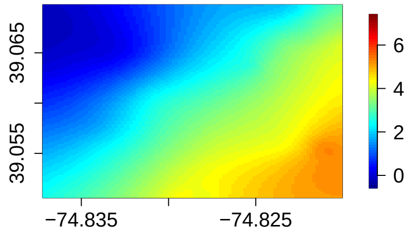
GWR Estimated Water Levels – Storm 2
