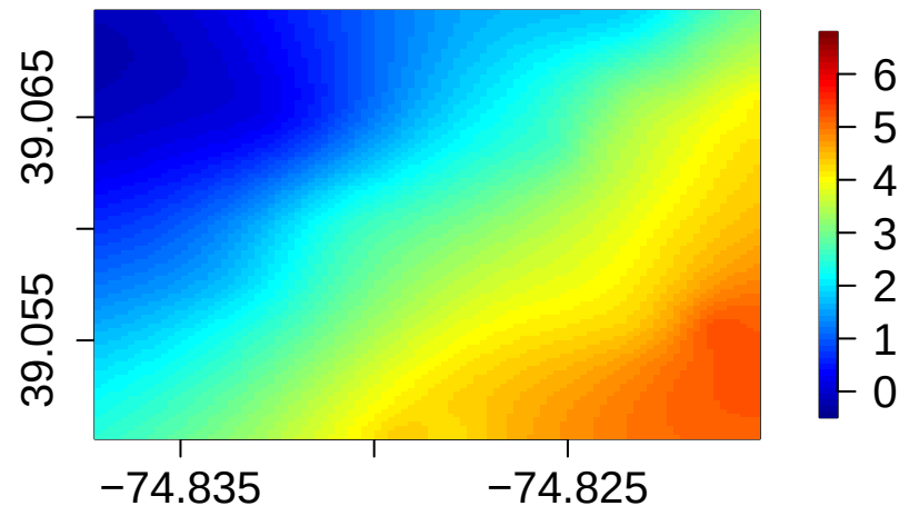
GWR Estimated Water Levels – Storm 6
