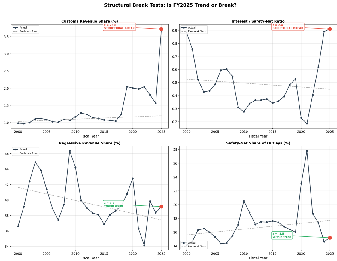
Figure 1: Departure-from-trend tests (4-panel: actual vs. trend)
