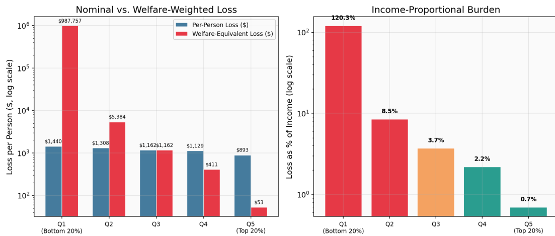
Figure 28: Welfare-weighted loss (log-scale, CRRA \sigma=2 )
