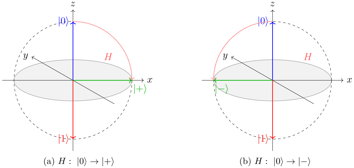
Figure 1.2: Bloch sphere representation of the Hadamard transformation
