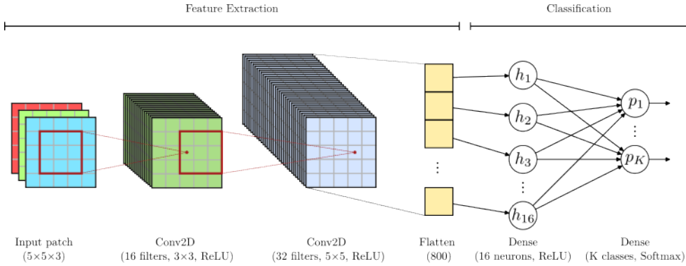
Fig. 4. CNN model structure.
