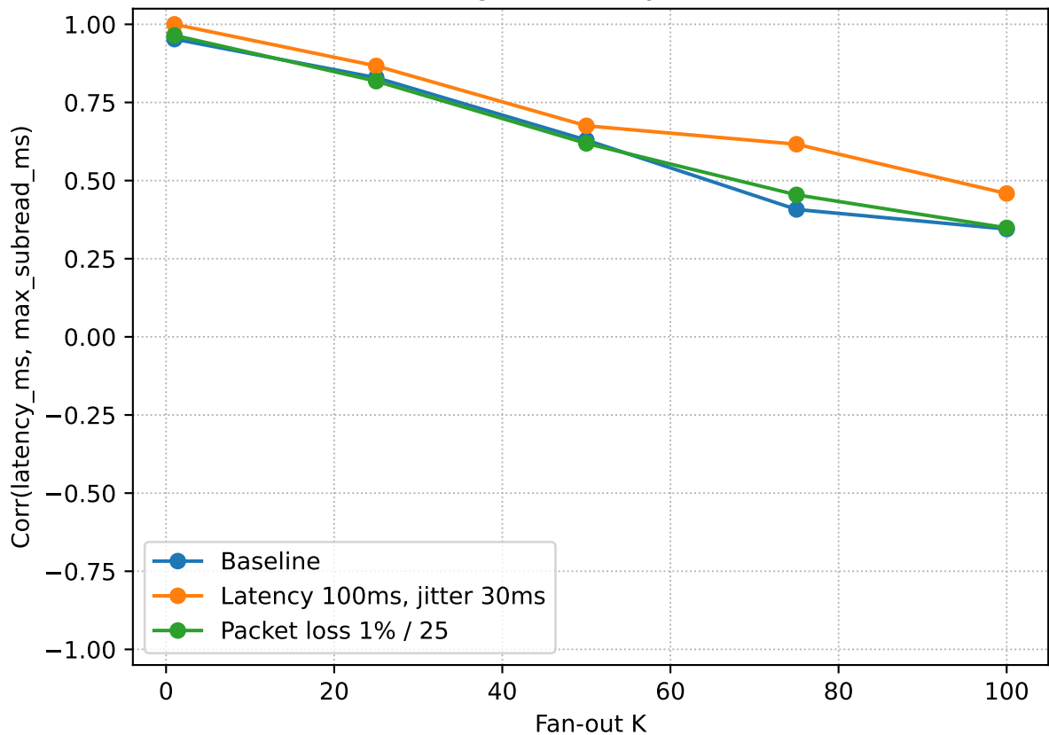
Correlation Between Logical Latency and Slowest Subread vs K
