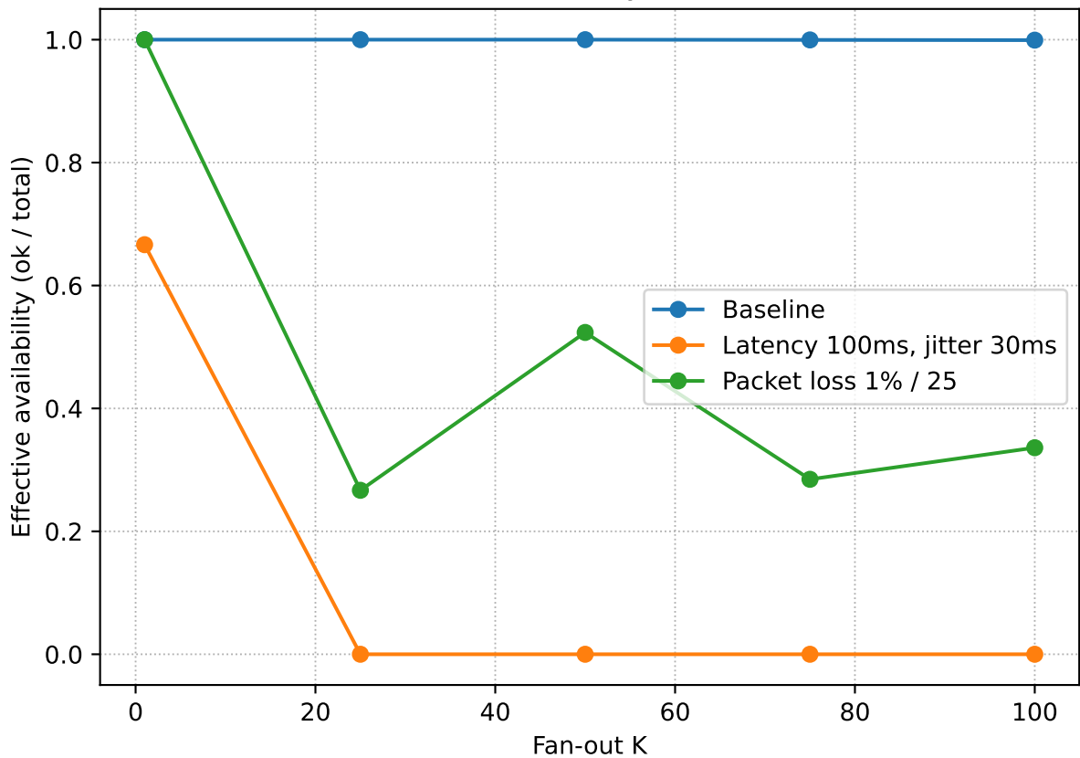
Effective Availability vs Fan-out K
