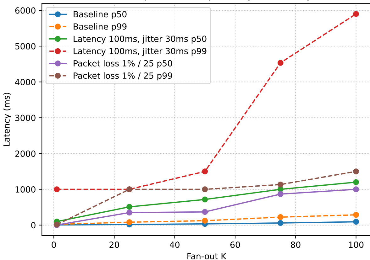
Median (p50) vs Tail (p99) Logical Latency
