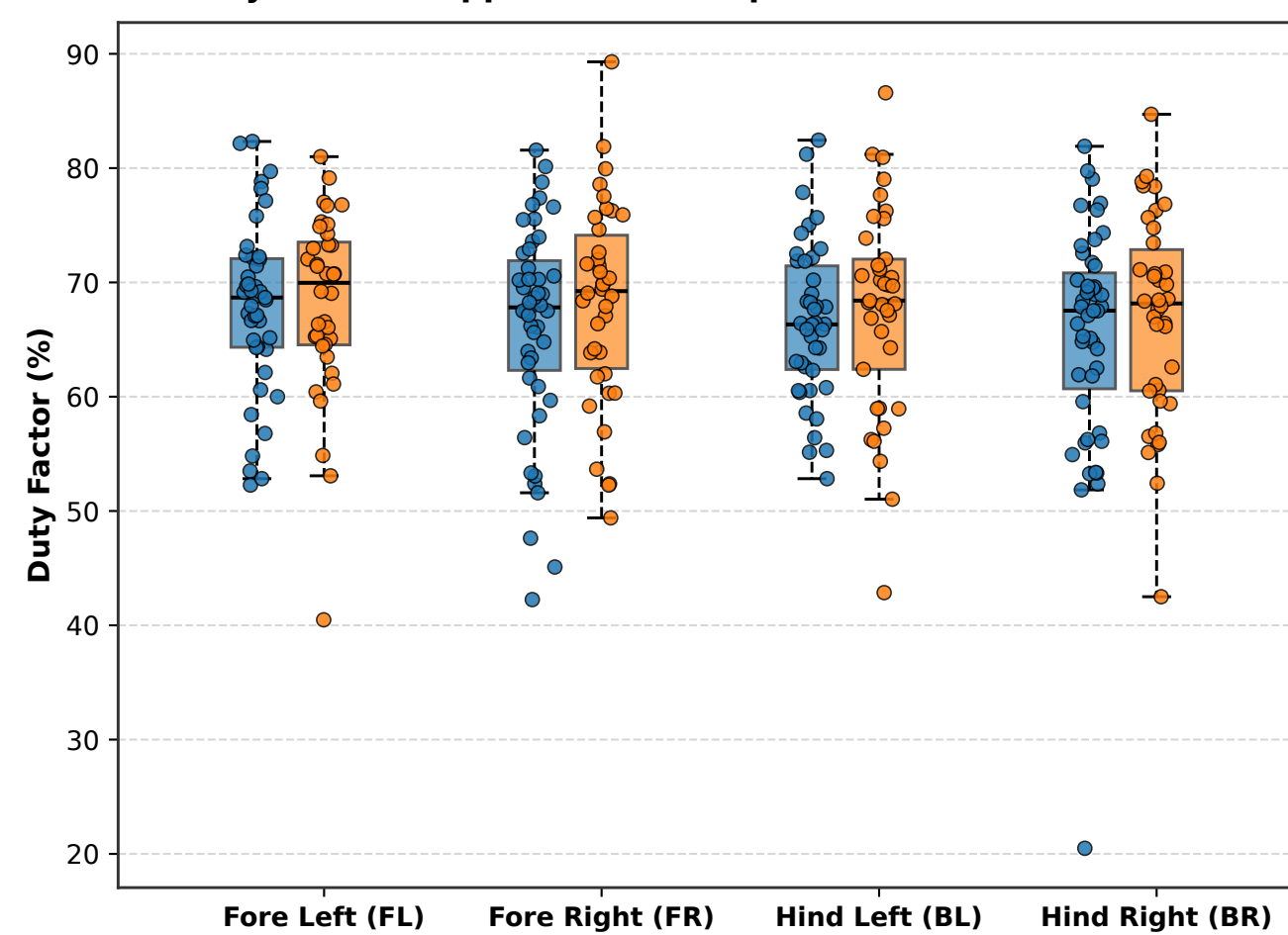
(C) Duty Factor (Support Phase Proportion)
