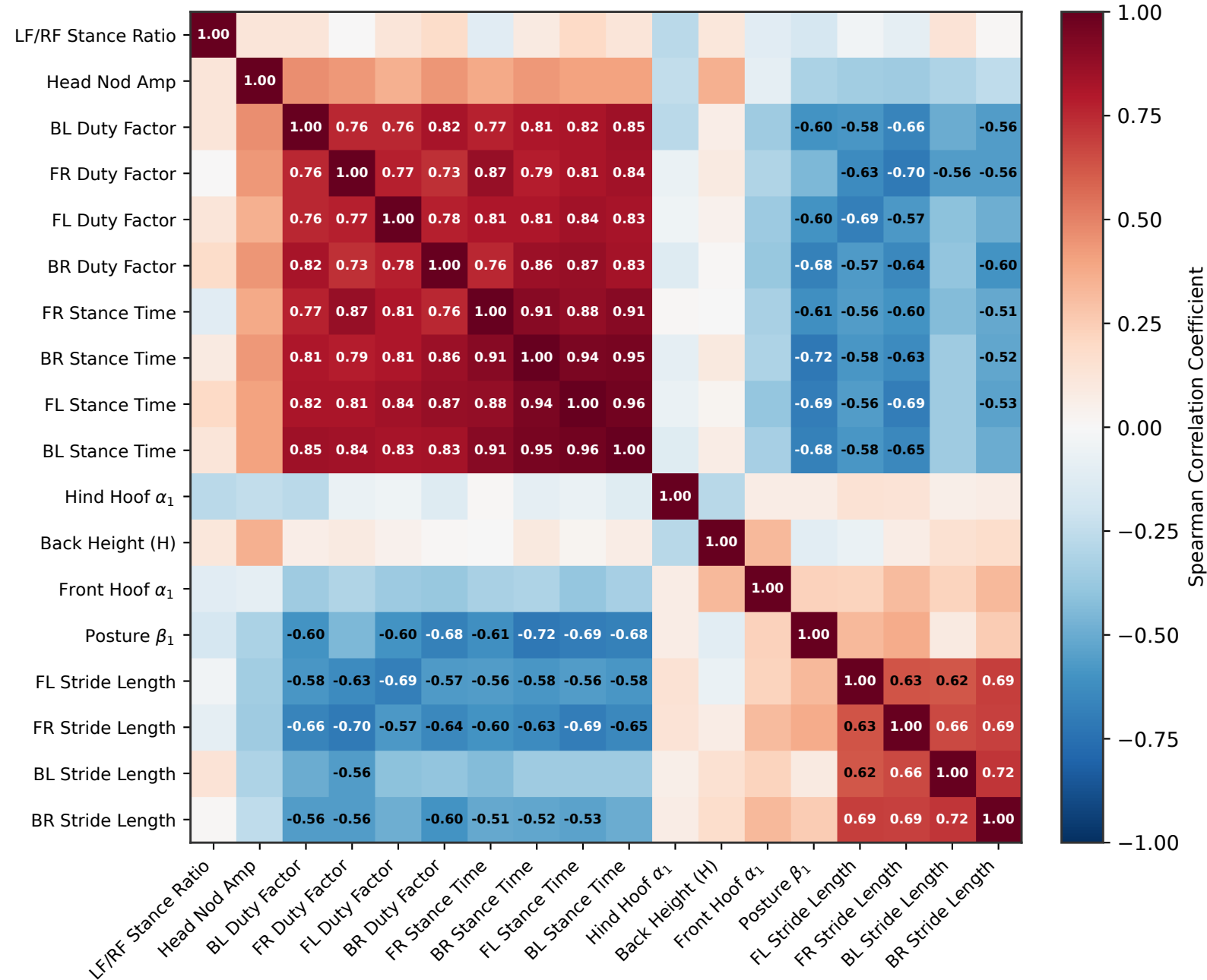
(A) Clustered Feature Correlation Matrix
