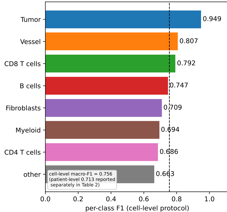
Frozen-feature phenotyping (Task 1)
